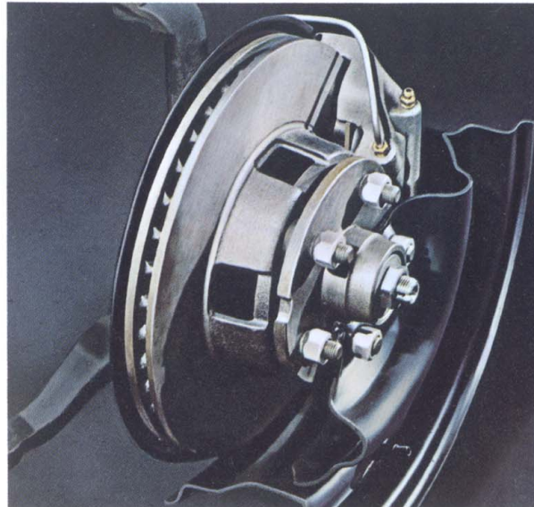
Front Disc Brakes
